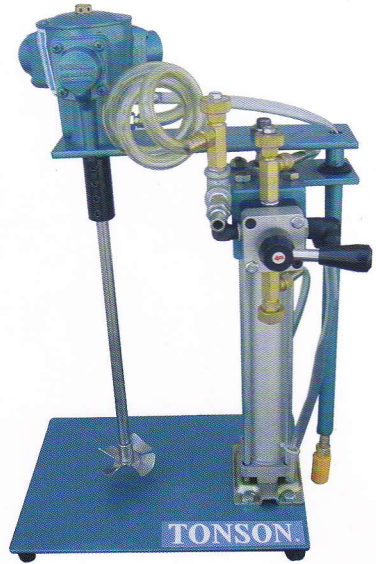
TS-LAU Laboratory Air Mixer • Entirely cylinder lift • operation easily • optional vane air motor
