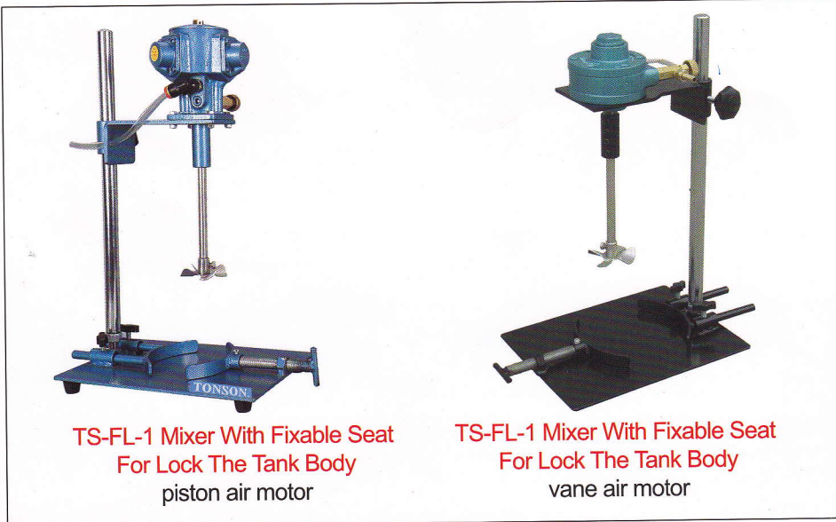
SUS Type And Steel Seat Can Be Customized. (Both For Piston And Vane)
