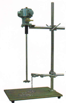
TS-FH-1 Mixer With Clamp
